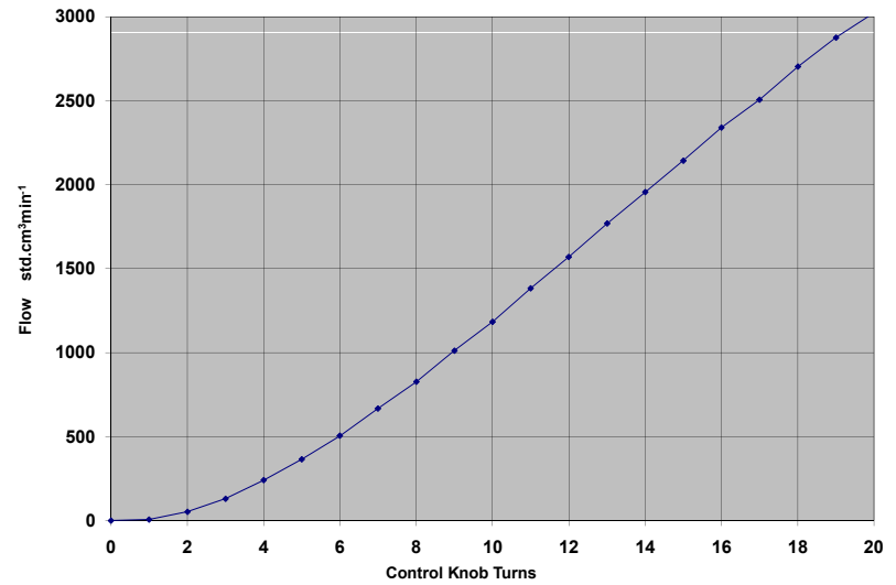
Typical Flow/Turns Plot for No. 3 Needle with 1bar differential Pressure
